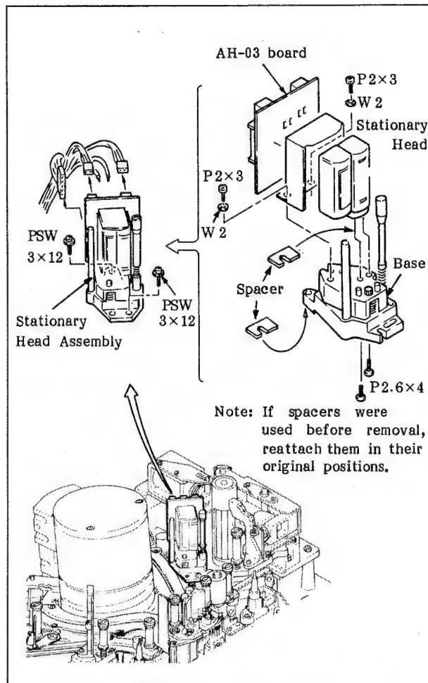
Fig. 6-125 Replacement of the Stationary Head
